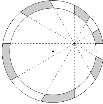
Figure 11: Thick crust with N = 6 and c \approx 6/7 .
