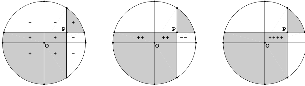
Figure 2: For N = 2 , gray minus white = 4 \times rectangle. Proof. Move signs from bottom to top, then from left to right.
