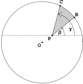
Figure 3: A slice: slice at P from \beta to \gamma = P\widehat{BC} .
