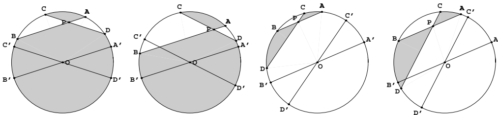
Figure 6: Opposing slices, remaining subcases.
