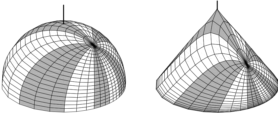
Figure 10: Hemisphere and cone calzones with N = 5 . The z -axis is shown poking through, to indicate the slice containing the center.
