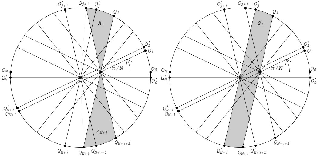
Figure 7: Opposing slices \widehat{PQ_j Q_{j+1}} and \widehat{PQ_{N+j} Q_{N+j+1}} . Figure 8: Strip \widehat{Q_j Q'_j Q'_{N+j} Q_{N+j}} .
