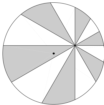
(a) Gray area equals white when N > 2 is even. (Here, N = 6 .)
