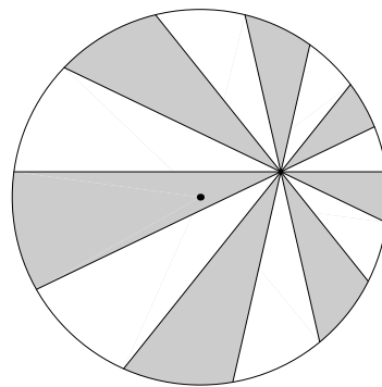
(b) Gray and white areas differ when N is odd. (Here, N = 7 .)
